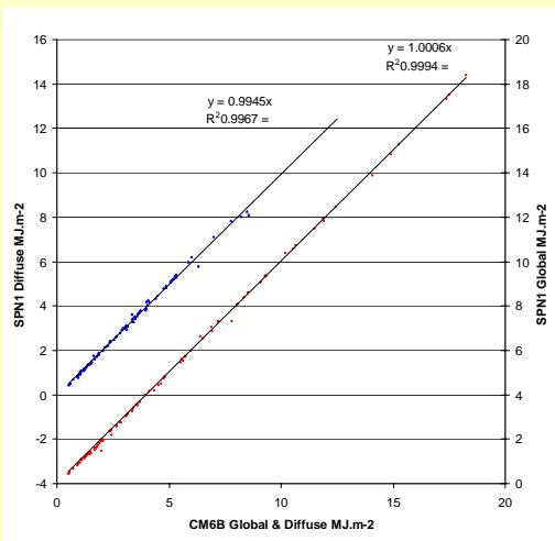
SPN1 Daily Integrals Global & diffuse compared with Kipp CM6B & tracking disk Sept – Dec 2004, daily integrals. (Note use of offset axes to make traces visible).
