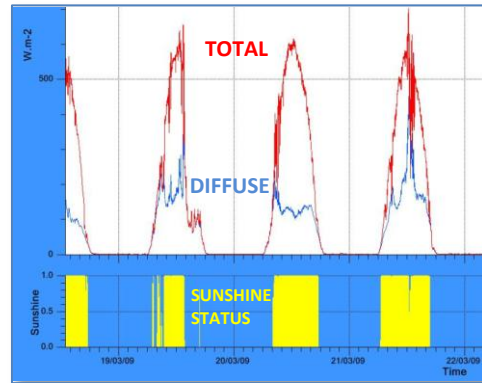
Figure 1 Graphical representation of the SPN1 readings logged over several days.
