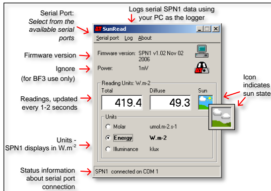
Figure 2 showing how SPN1 real-time readings appear on a PC running the SunRead program
