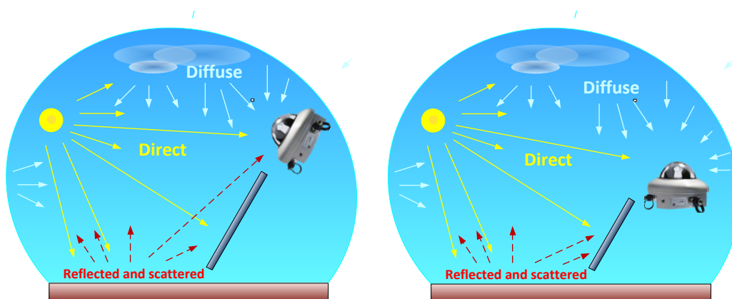
Figure 5: Schematic diagram illustrating the behaviour of a tilted and horizontal SPN1s. The SPN1 sees everything above its horizon. Tilting an SPN1 can be particularly useful for recording the same diffuse radiation as that received by a tilted photovoltaic panel (provided it does not see two suns – which may cause unreliable readings). A horizontal SPN1 can be useful for ease of calculating the DNI – Direct Normal Irradiance (if you don't have a sun tracking device).
