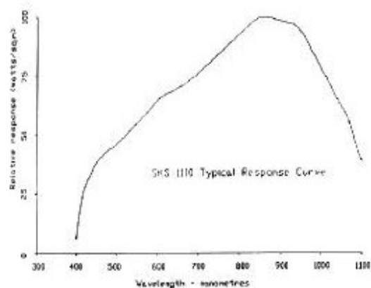
Pyranometer-Sensor SKS1110 (W/m 2 )
