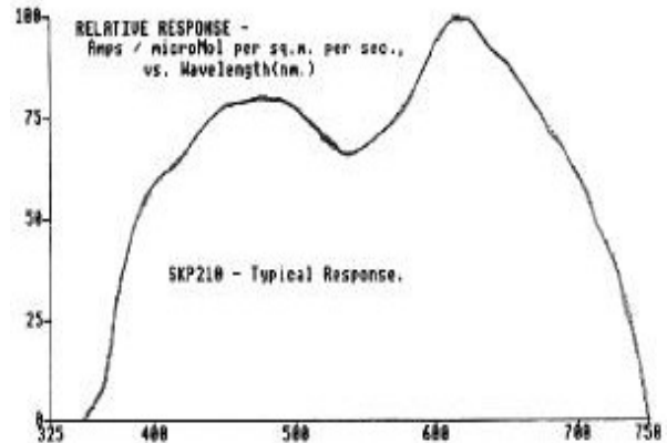
PAR-«special»-Sensor SKP210
