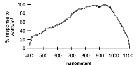
PYRANOMETER SKS 1110
