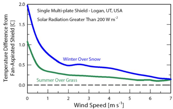
Effect of Wind Speed on Multi-plate Shields
