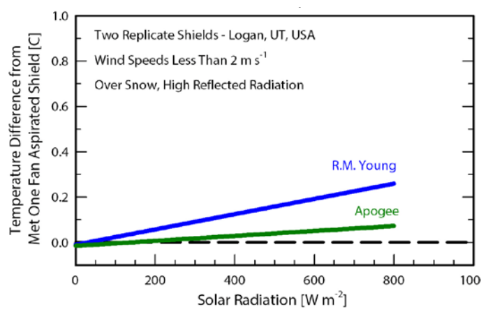
Wintertime Performance of Fan-aspirated Radiation Shields
