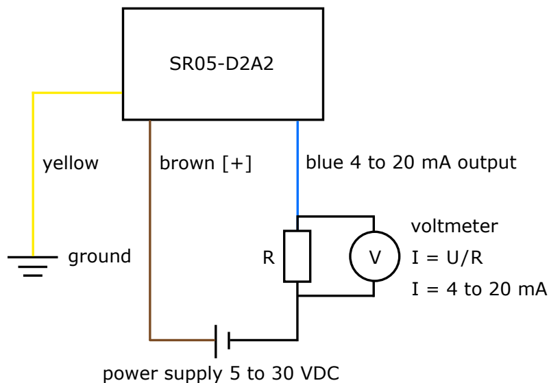
Figure 5.8.2 Electrical diagram of the connection of SR05-D2A2 to a typical voltmeter or datalogger with the capacity to measure voltage signals. Usually a 100 \Omega shunt resistor ( R ) is used to convert the current to a voltage. SR05-D2A2 operates on a supply voltage of 5 to 30 VDC.
